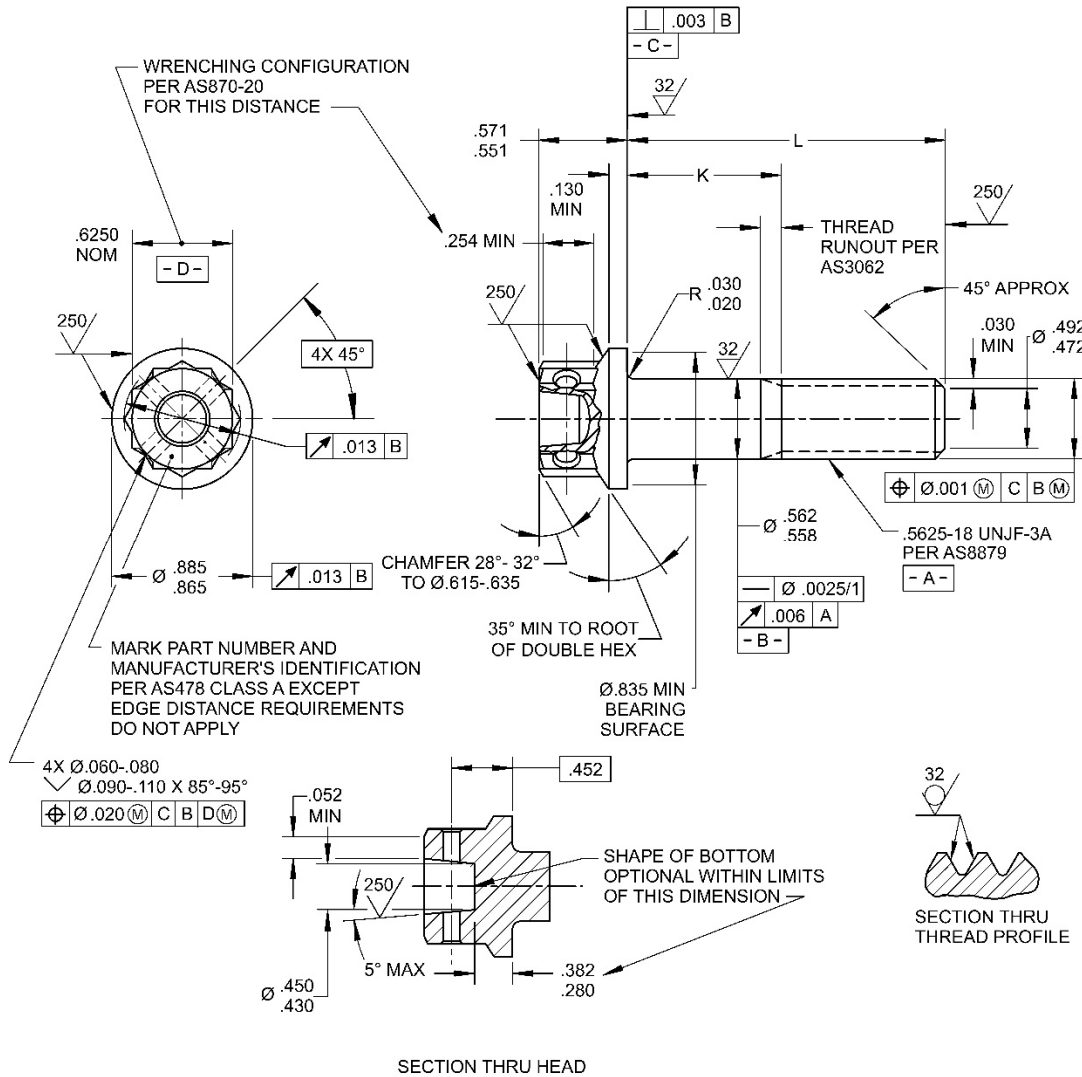
FIGURE 1 - BOLT
